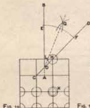
Fig. 10. Method of drawing octagons in contact by sides.
