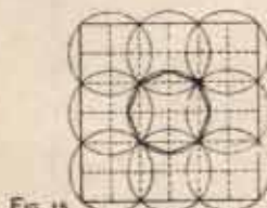
Fig. 15. Method of drawing overlapping octagons.
