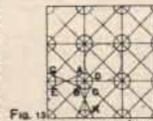
Fig. 13. Method of drawing octagons in contact by their angles.
